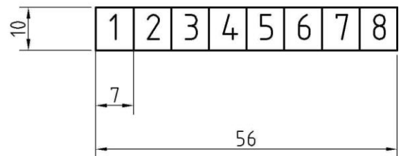
Place for marking. Height of letters 6mm
